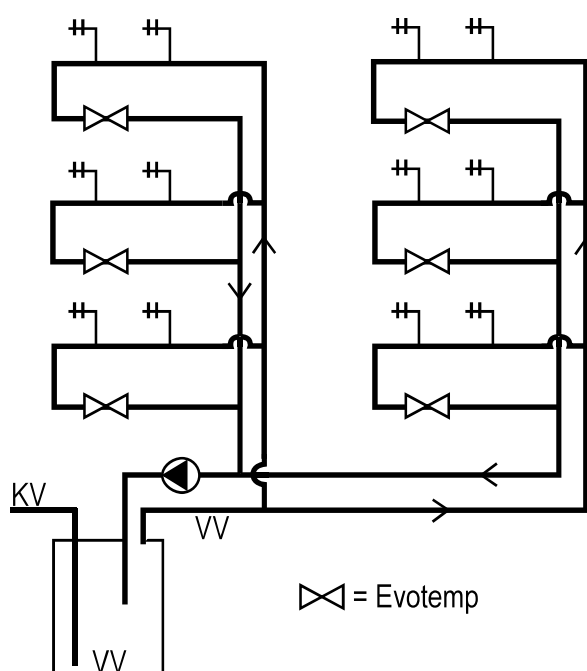
Kopplingsschema/Wiring diagram
