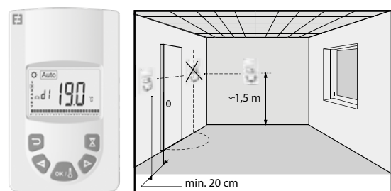
Abb. 97 Funk-Raumthermostat
