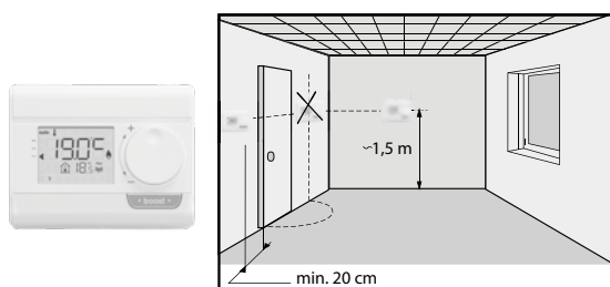
Abb. 102 Funk-Raumthermostat
