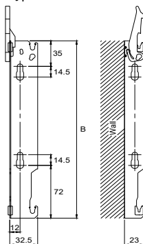
Bracket Type 11
