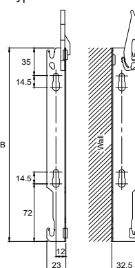
Bracket Type 22
