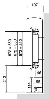
LST type 11 elevation
