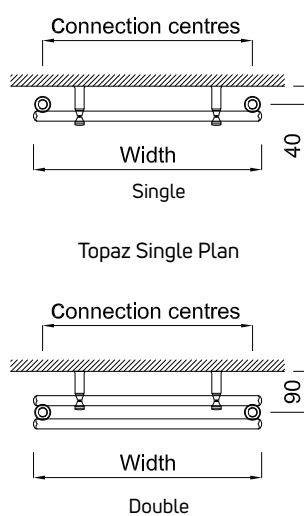
Topaz Double Plan
