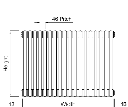
Forza Horizontal Elevation
