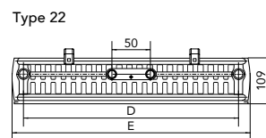
Compla Vertical Plan
