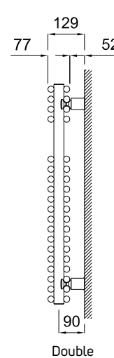
Topaz Double Section
