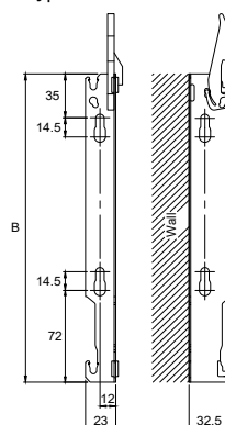
Bracket Type 22
