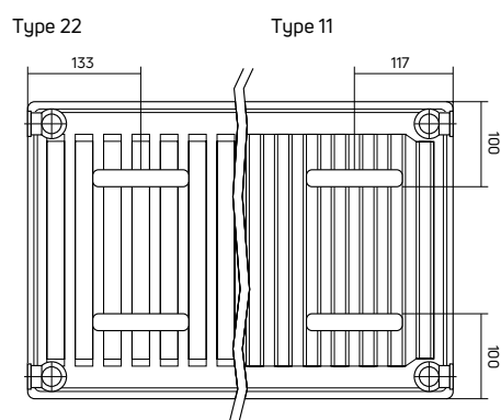
Bracket Type 11
