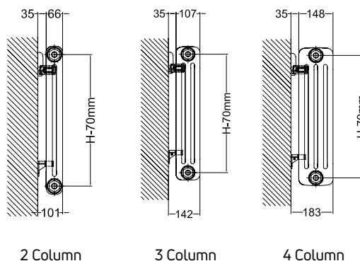
Forza Horizontal Section
