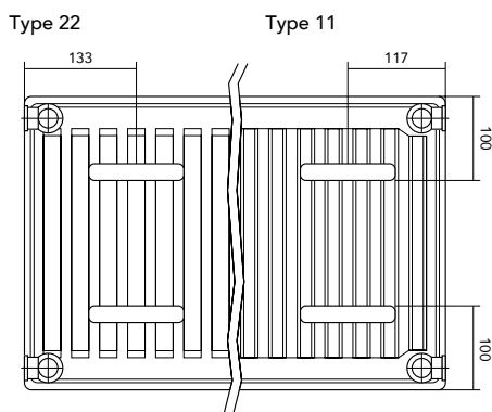
Bracket Type 11
