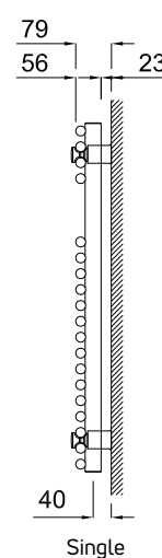
Topaz Single Section
