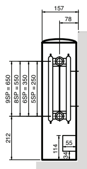
LST type 22 side elevation
