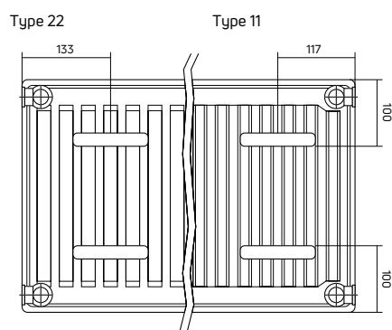
Bracket Type 11
