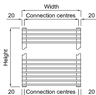
Pearl Elevation
