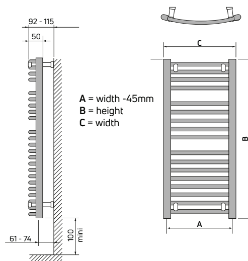
Flores curved
