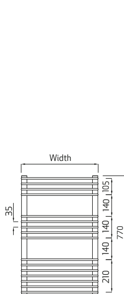
Pearl 770 High
