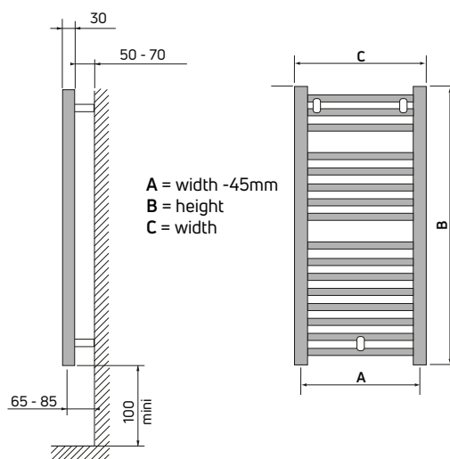
Flores straight
