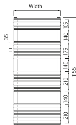
Pearl 1155 High
