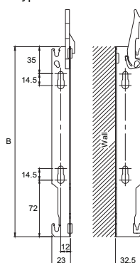
Bracket Type 22
