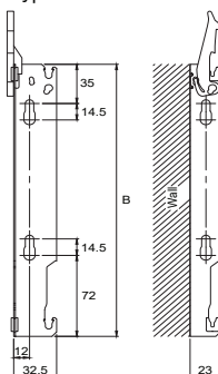
Bracket Type 11
