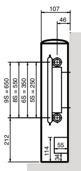
LST type 11 elevation
