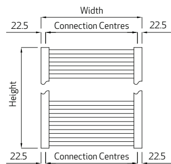
Crystal Elevation
