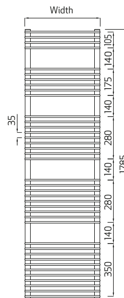
Pearl 1785 High
