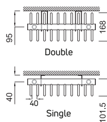
Adagio 70 Vertical Plan
