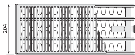
PURMO FCV 44
