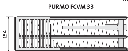
PURMO FCVM 33
