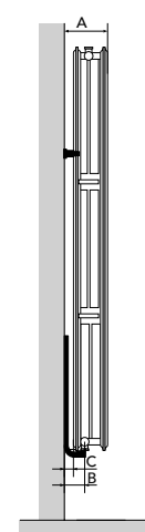
Type 22 Ligna Vertical Section
