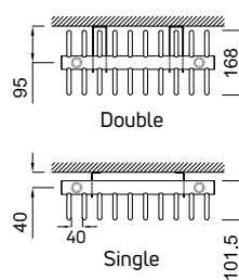
Adagio 70 Vertical Plan
