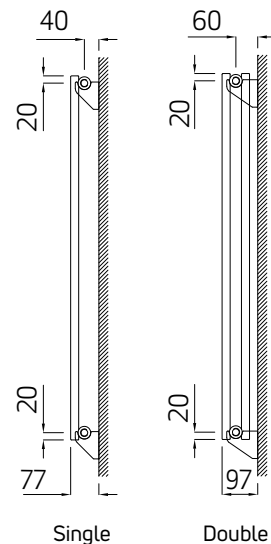
Plaza Vertical Section
