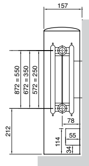
LST type 22 side elevation
