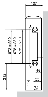
LST type 11 elevation
