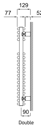
Topaz Double Section
