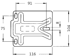
Dimensions of base-plate for Floor Bracket SK
