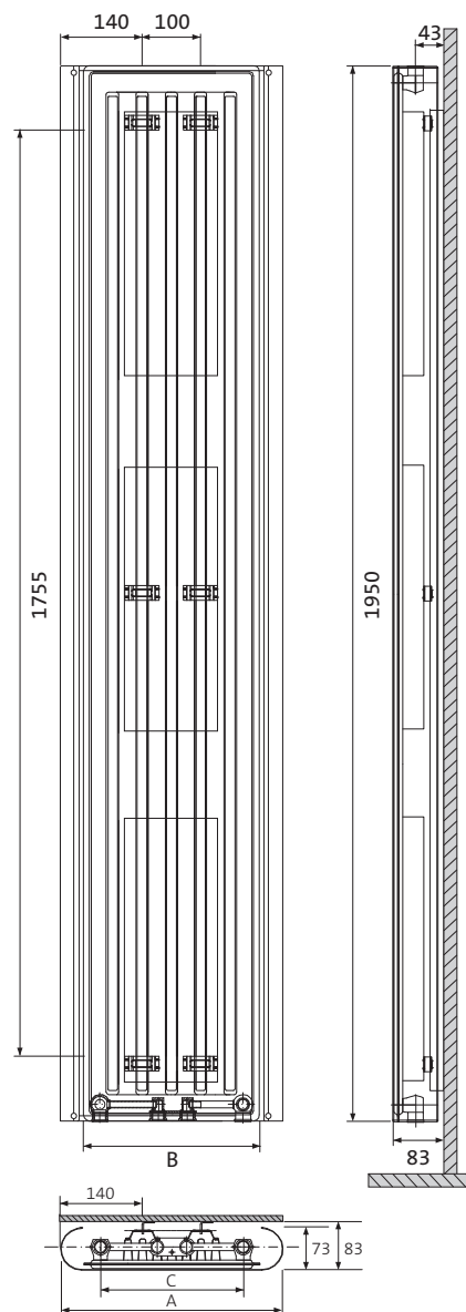
TYPE 11 (380)
