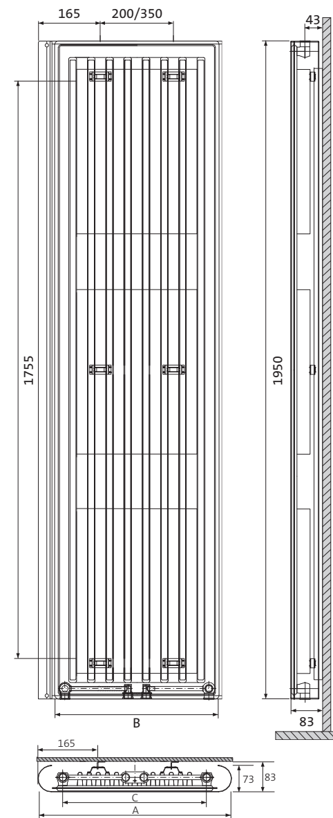
TYPE 11 (530/680)
